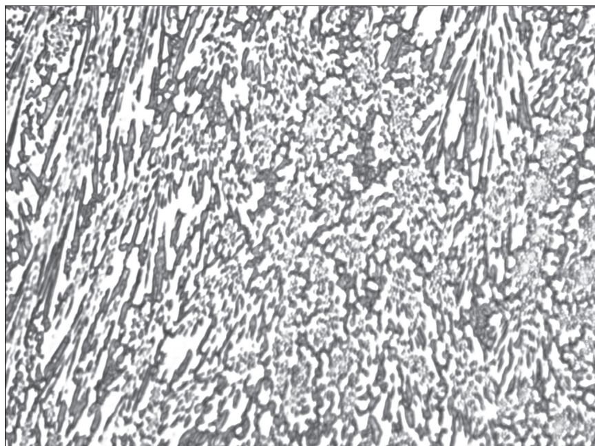
Optical micrograph of a Soonv ® 1 weld overlay
