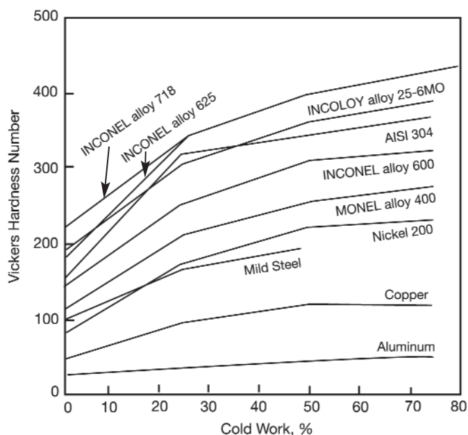
Figure 6 - The work-hardening rate for SOONV alloy 25-6MO is similar to that for AISI 304 stainless steel.
