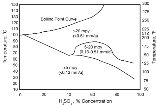
Figure 4 - Isocorrosion chart for SOONV alloy 25-6MO in sulfuric acid.
