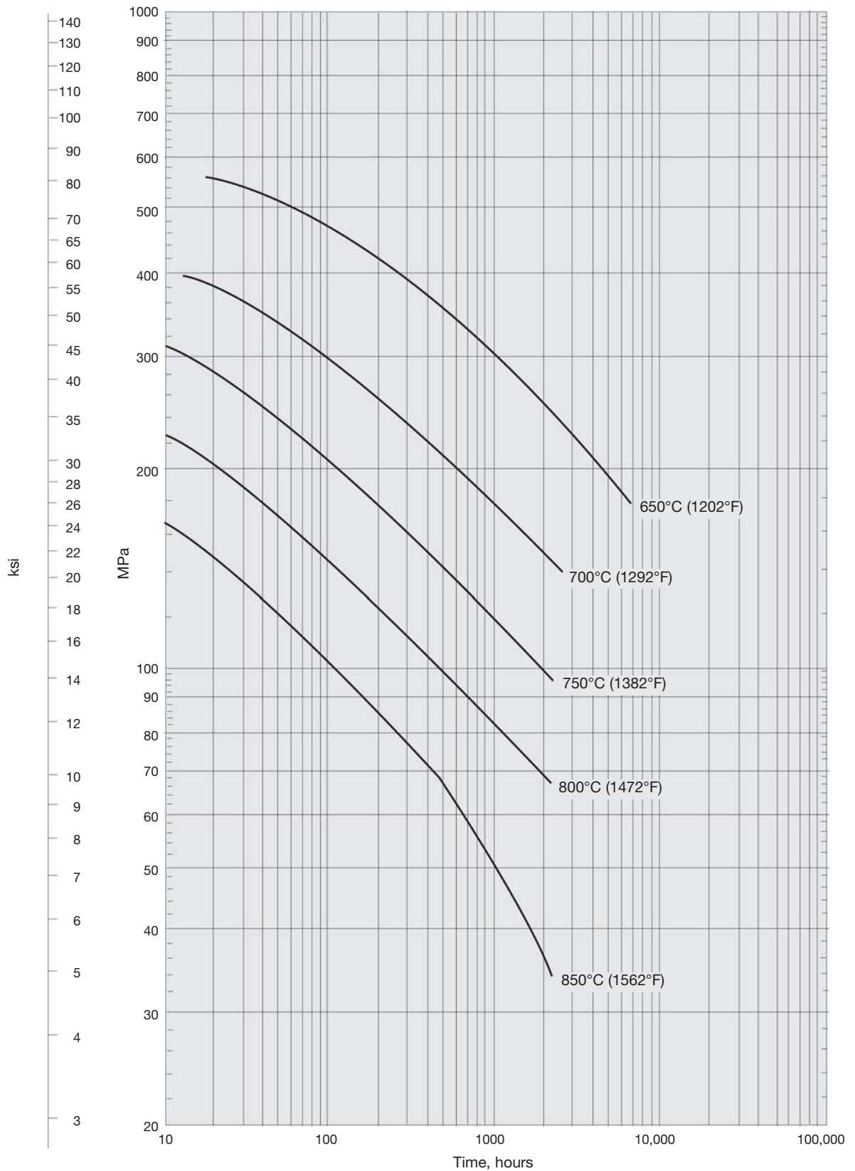
Figure 15 . Creep-rupture properties of SOONV alloy 80A cold rolled sheet, 1.6 mm (0.06 inch) thick. Results from 1 cast.
