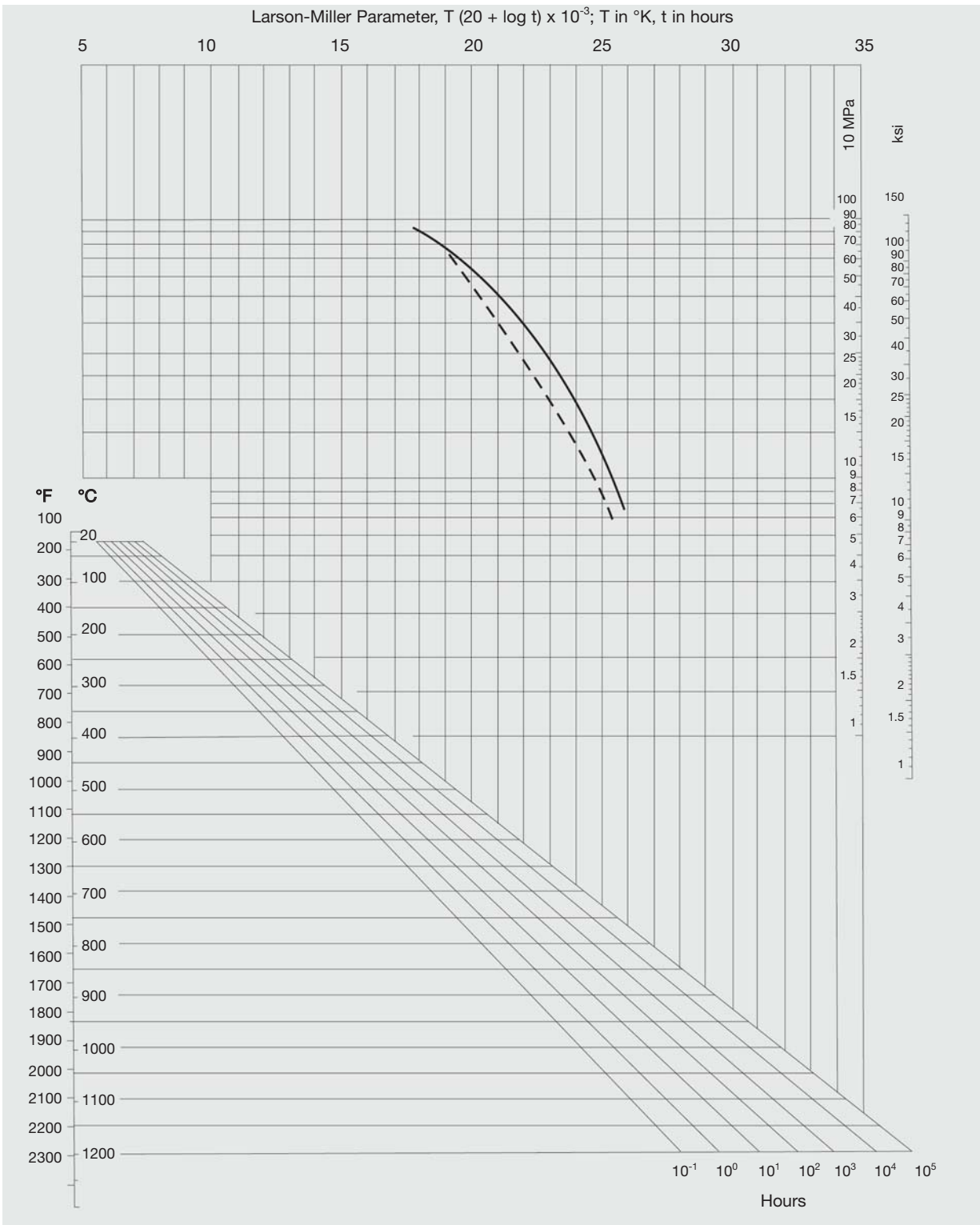
Figure 13. Creep rupture properties of SOONV alloy 80A bar and sheet.
