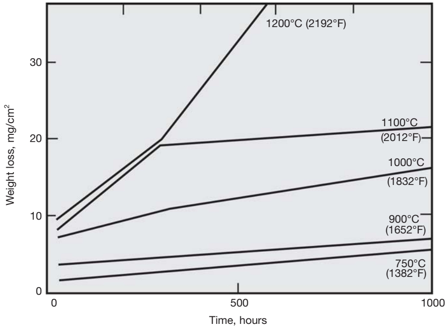
Figure 26. Isothermal oxidation resistance of SOONV alloy 80A.
