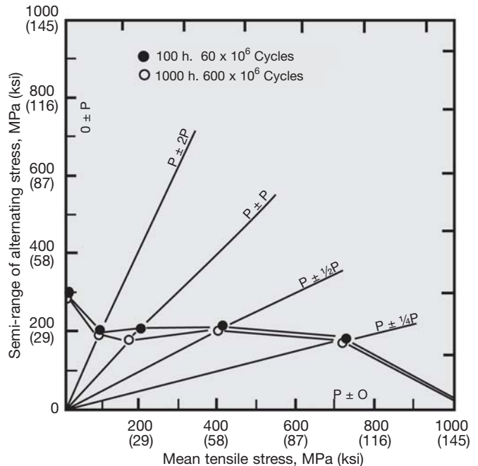
Figure 18. Fatigue test at 480°C (896°F)
