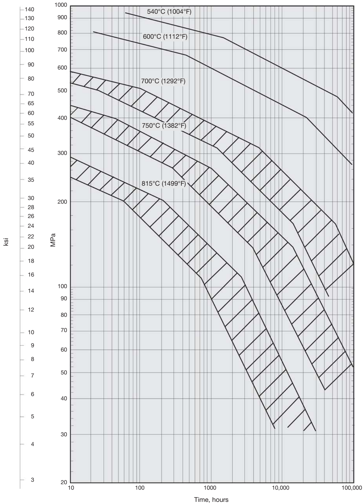
Figure 12 . Creep properties of SOONV alloy 80A extruded bar, subsequently forged. Heat treatment 8 hours/1080°C (1976°F)/air cooled + 16 hours/700°C (1292°F)/air cooled. 98% confidence region on 16-18 casts.
