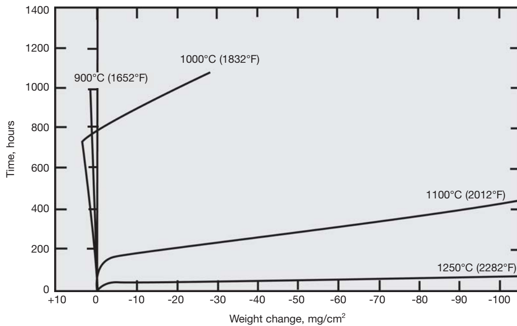
Figure 27. Cyclic oxidation resistance of SOONV alloy 80A. (20 minutes in furnace, 10 minutes in air.)
