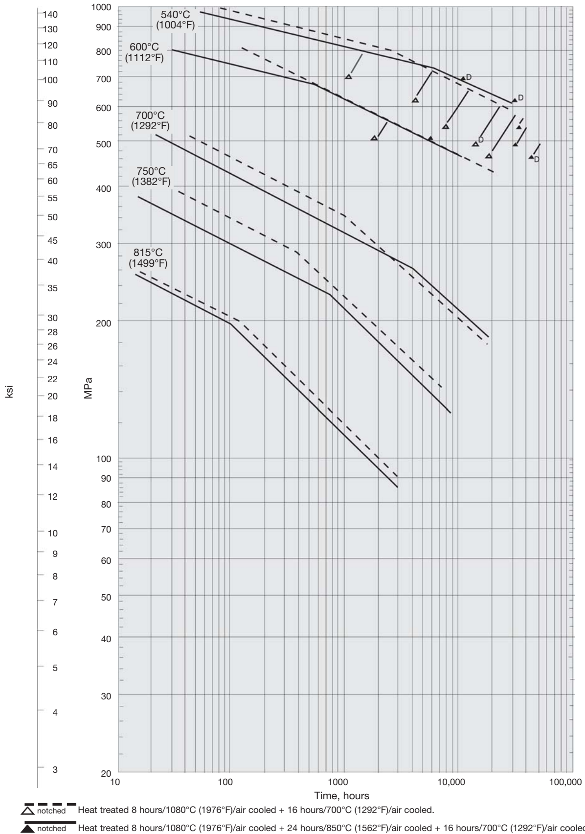
Figure 14 . Creep properties of SOONV alloy 80A extruded section, subsequently cold rolled. Average results from 5 casts.
