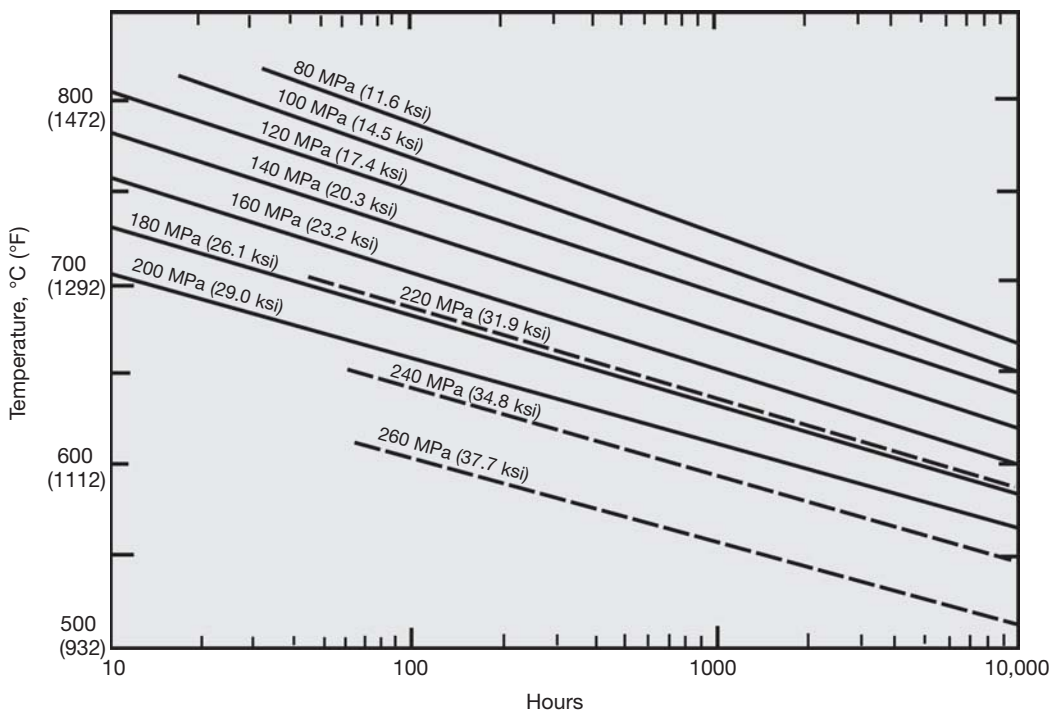
Figure 23. Stress relaxation properties of SOONV alloy 80A.
