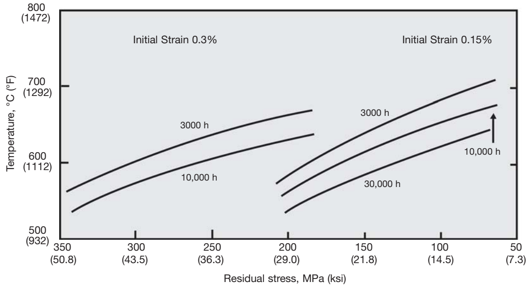
Figure 25. Relationship between initial strain, residual stress and time. SOONV alloy 80A, heat treated 8h/1080°C (1976°F)/air cooled + 16h/700°C (1292°F)/air cooled.
